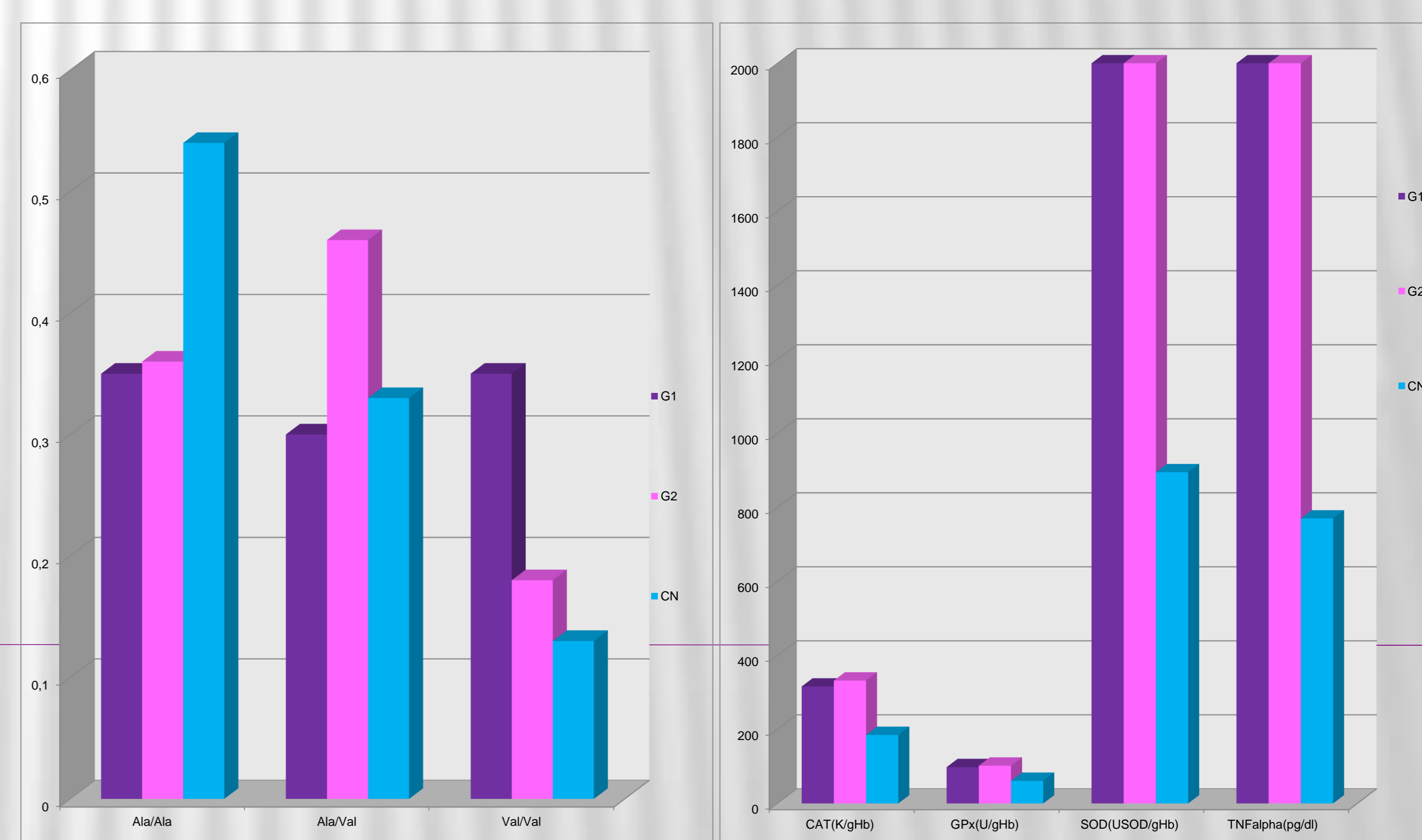
Graph I. SOD-Mn Ala9Val FG.
